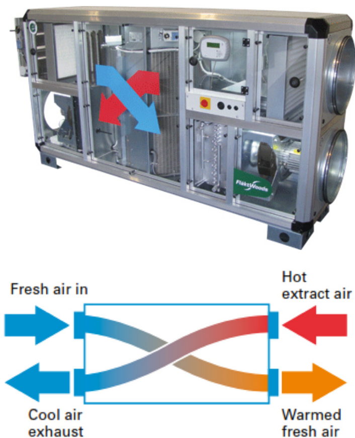
Figure 1. Heat Recovery Ventilator 2
