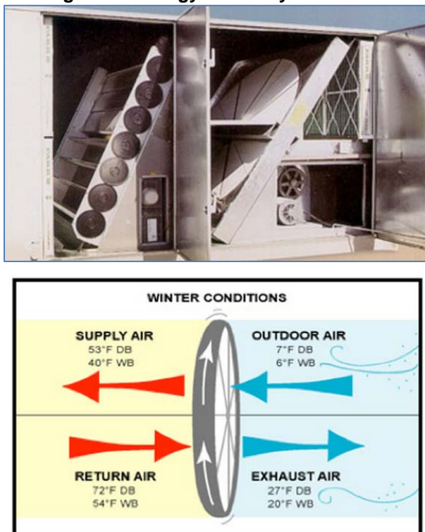
Figure 1: Energy Recovery Ventilator 3
