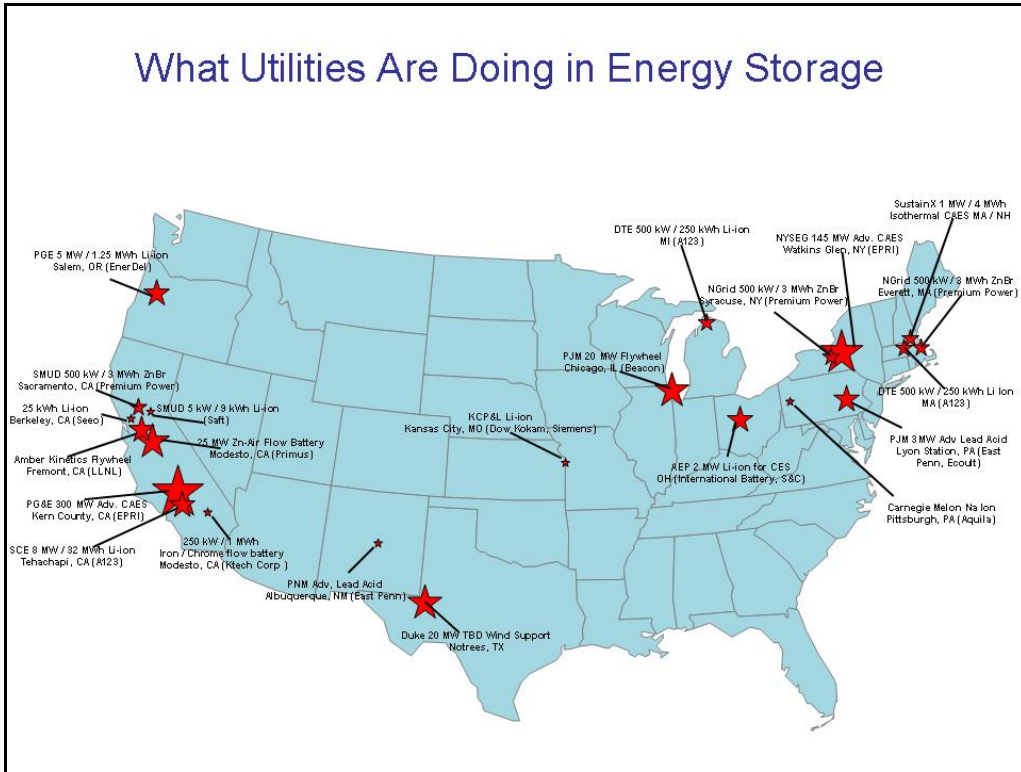
Figure ES-3 ARRA-Funded Utility Energy Storage Projects
