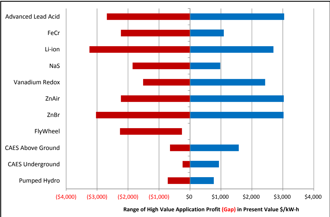
Figure 5-2 Gap Chart by Technology Including All Applications
